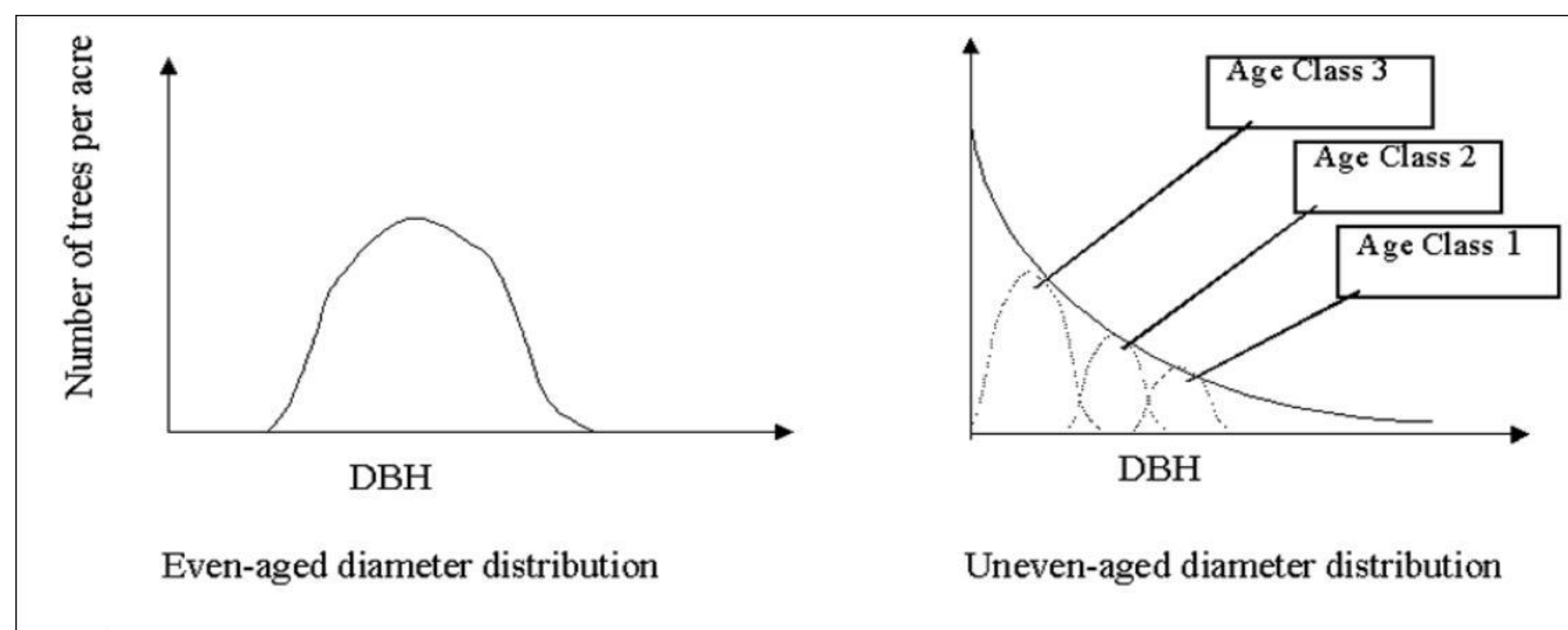
Figure 2. Diameter distribution in even-aged and uneven-aged forests
