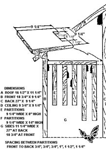
Figure 9. Bat roosting box.
